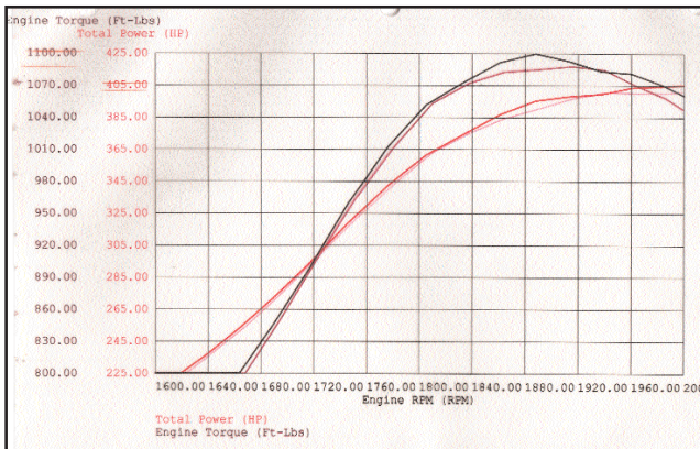
Dyno Chart: 1998 Dodge Ram
