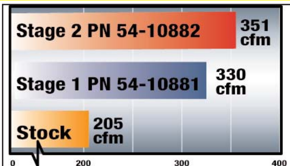
Airflow Comparison (CFM) @ 1.5" H 2 O
